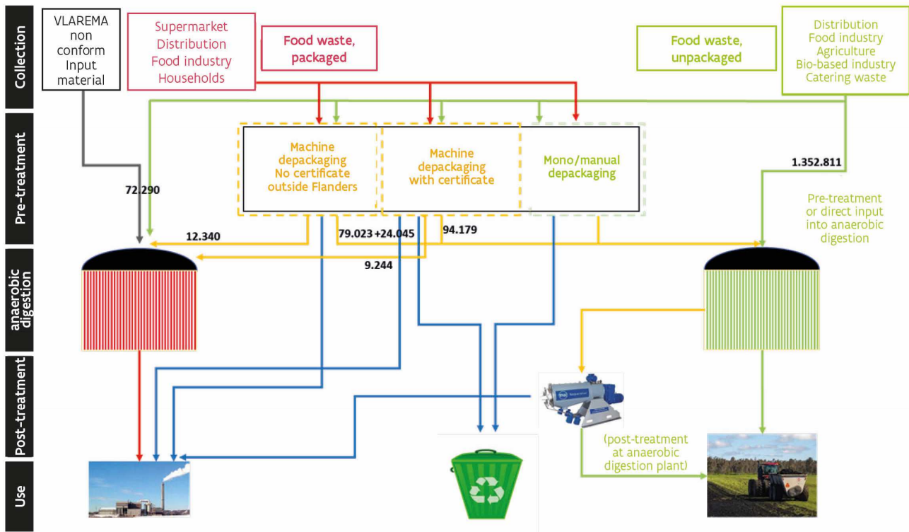
Figure 5: Schematic overview of quantities of separately collected and processed food waste, including food and kitchen waste in Flanders in 2020 (in tonnes)
