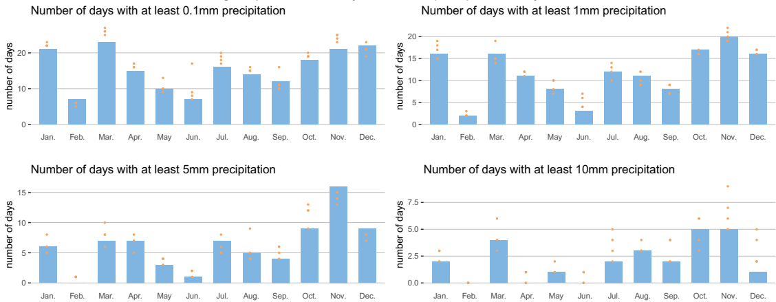
Zvevegem plu19a, monthly number of precipitation days in 2023
