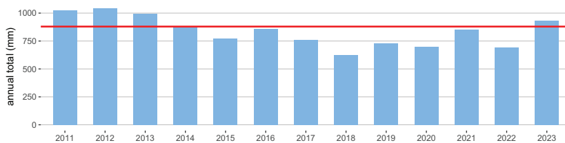
Time series of annual precipitation totals (blue bars) versus the climate normal 1991–2020 (horizontal line, 879mm)
