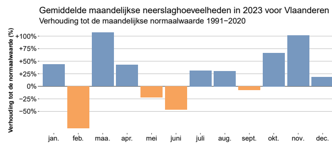
Figure 3: Monthly precipitation anomalies with respect to the period 1991-2020 on average for the Flemish Region from January to December 2023.
