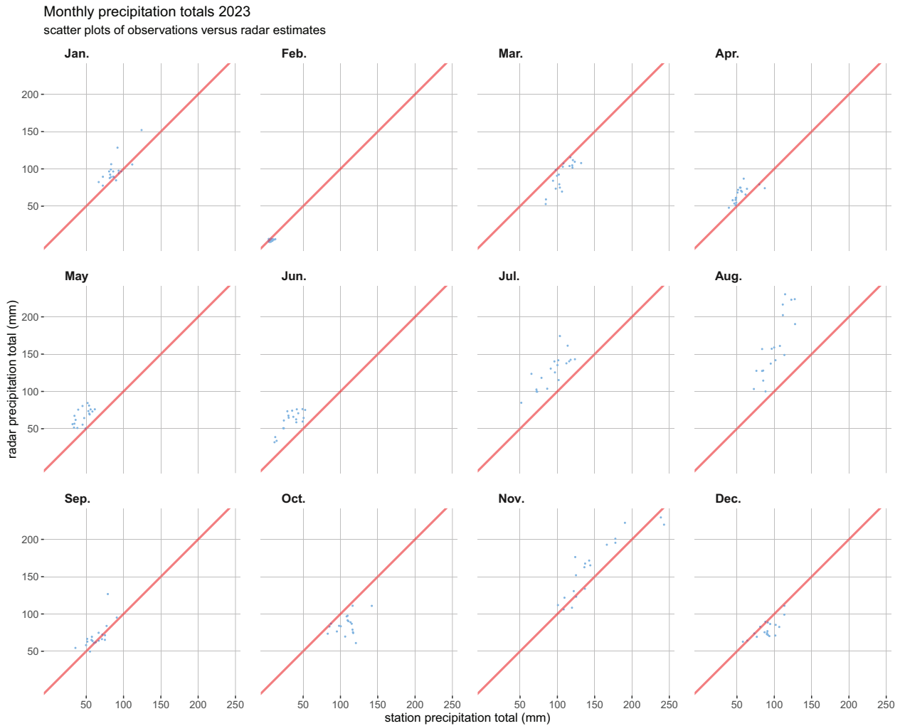
Figure 15: Scatter plots of the monthly totals of the HIC stations versus radar-derived estimates.
