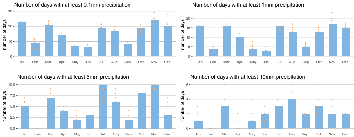
Zoutleeuw plu18a, monthly number of precipitation days in 2023
