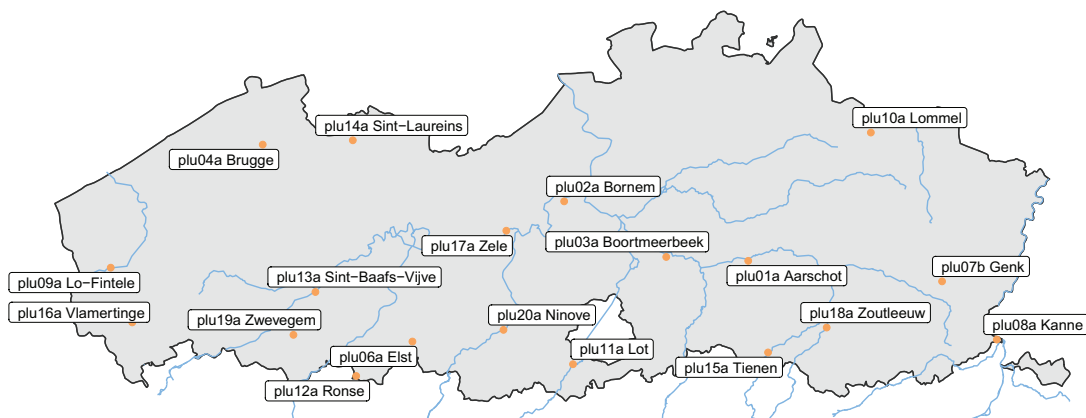
Figure 5: Location of the operational HIC rain gauges in 2023.
