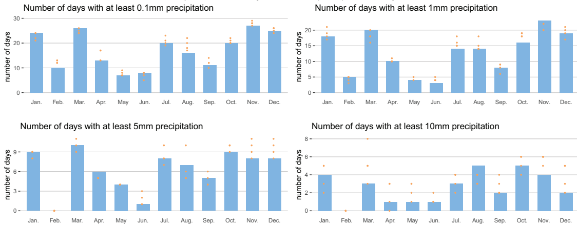
Lommel plu10a, monthly number of precipitation days in 2023
