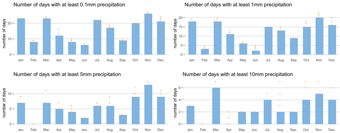
Ninove plu20a, monthly number of precipitation days in 2023
