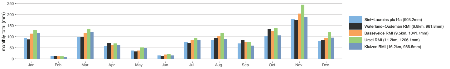
Sint-Laureins plu14a monthly precipitation totals in 2023
