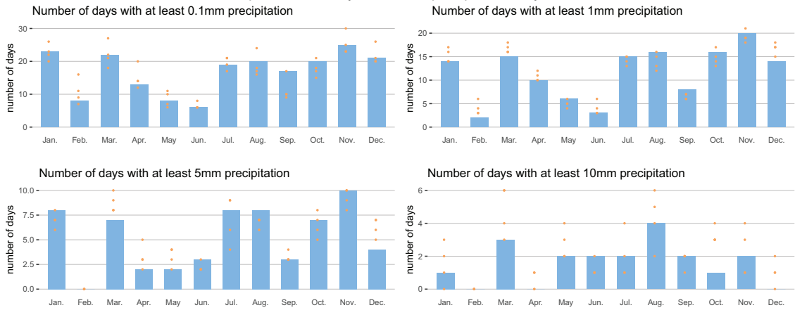
Tienen plu15a, monthly number of precipitation days in 2023
