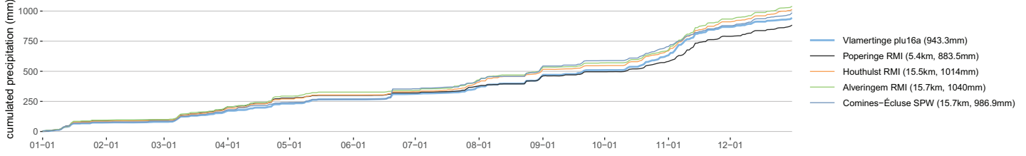
Vlamertinge plu16a cumulative precipitation in 2023
