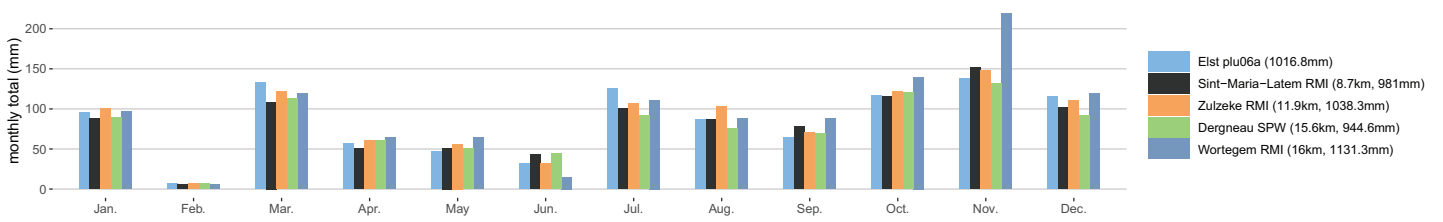
Elst plu06a monthly precipitation totals in 2023
