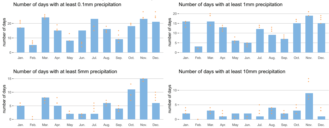
Vlamertinge plu16a, monthly number of precipitation days in 2023
