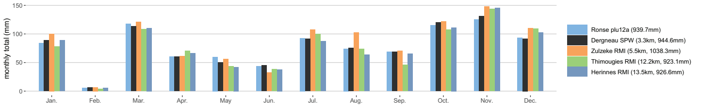
Ronse plu12a monthly precipitation totals in 2023
