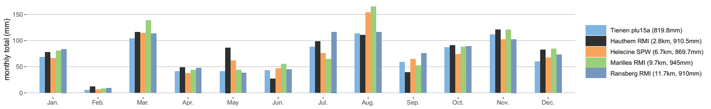
Tienen plu15a monthly precipitation totals in 2023
