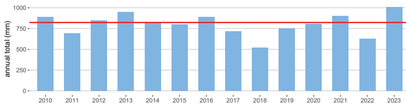
Elst plu06a Time series of annual precipitation totals (blue bars) versus the climate normal 1991–2020 (horizontal line, 823mm)
