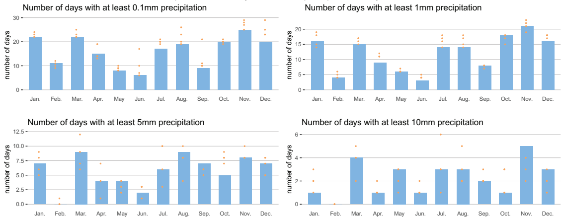
Kanne plu08a, monthly number of precipitation days in 2023
