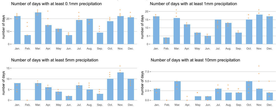
Elst plu06a, monthly number of precipitation days in 2023
