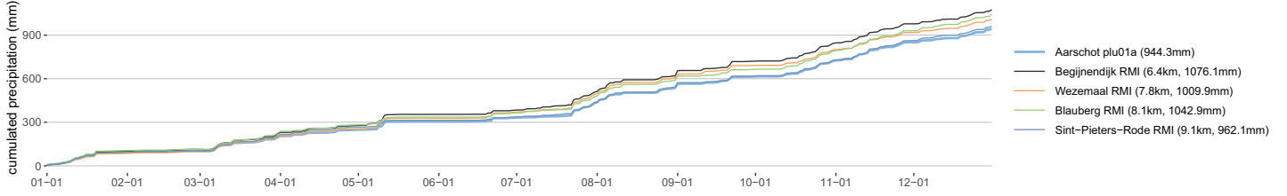
Aarschot plu01a cumulative precipitation in 2023
