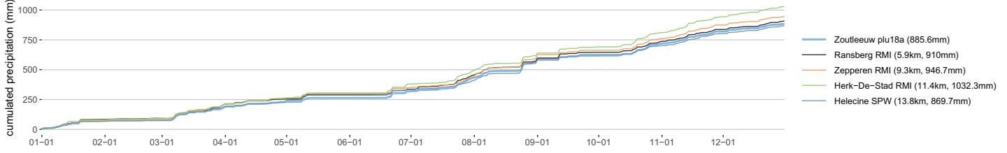
Zoutleeuw plu18a cumulative precipitation in 2023
