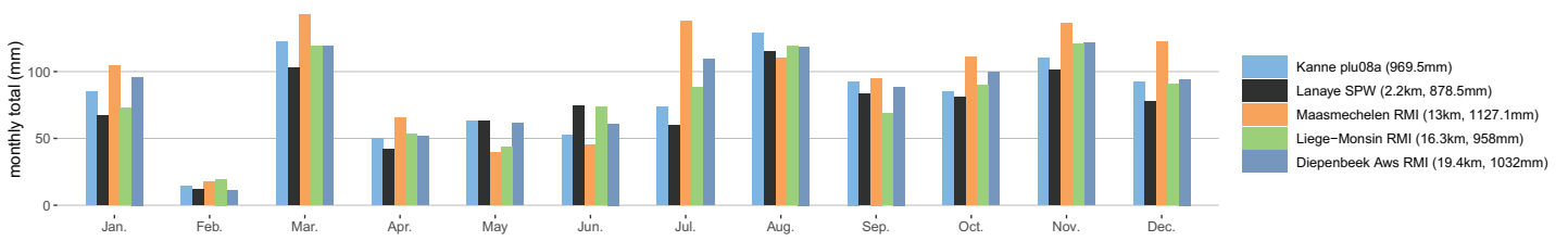
Kanne plu08a monthly precipitation totals in 2023
