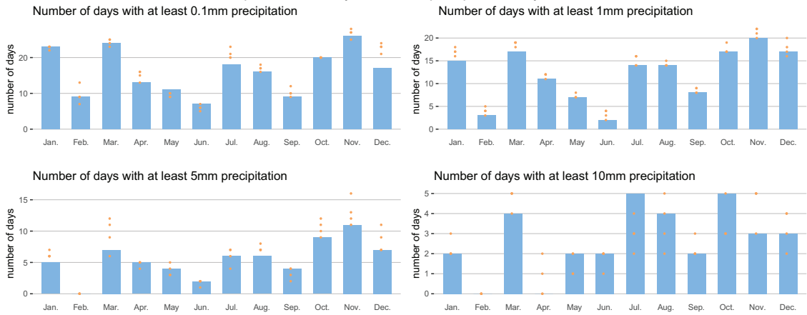
ZeZe plu17a, monthly number of precipitation days in 2023
