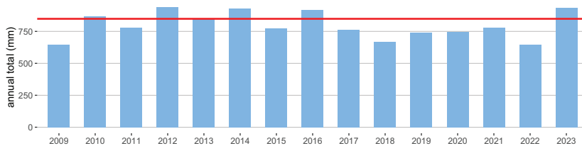
Time series of annual precipitation totals (blue bars) versus the climate normal 1991–2020 (horizontal line, 848mm)
