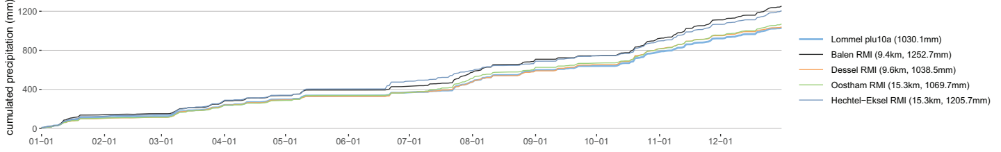
Lommel plu10a cumulative precipitation in 2023
