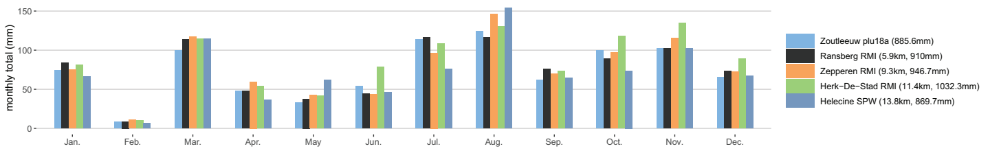
Zoutleeuw plu18a monthly precipitation totals in 2023
