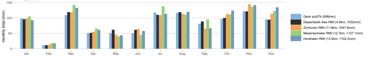
Genk plu07b scatter plot of daily precipitation totals
