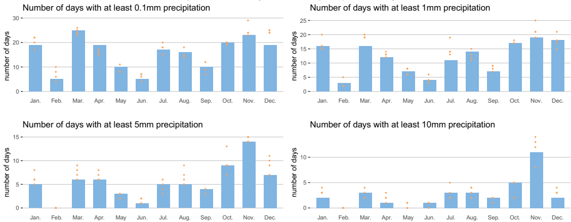
Lo-Fintele plu09a, monthly number of precipitation days in 2023
