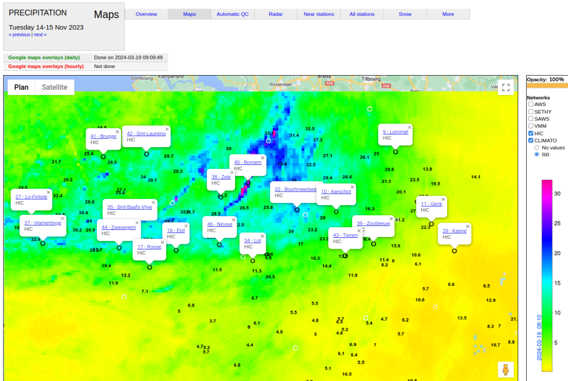
Figure 7: Data visualisation on maps in PluvioControl: comparison against daily radar data (case of November 14, 2023). The background field represents the estimations of the radar of Jabbeke. The numbers correspond to the observations of the climatological stations.
