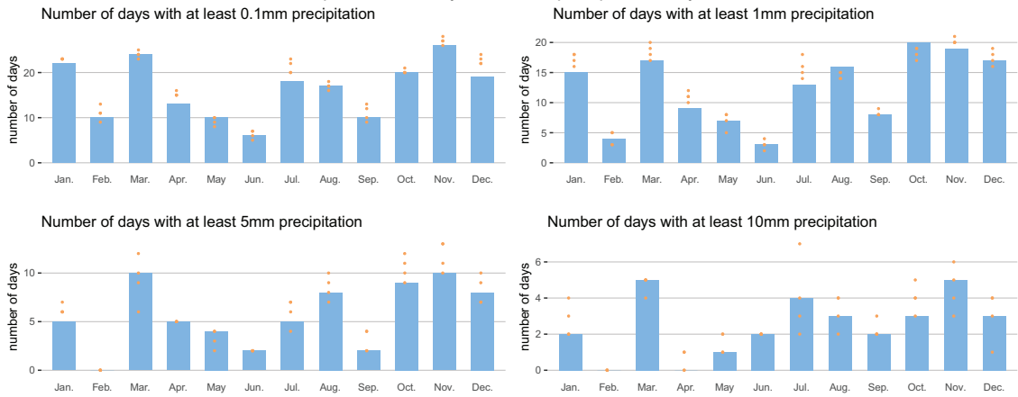
Bornem plu02a, monthly number of precipitation days in 2023
