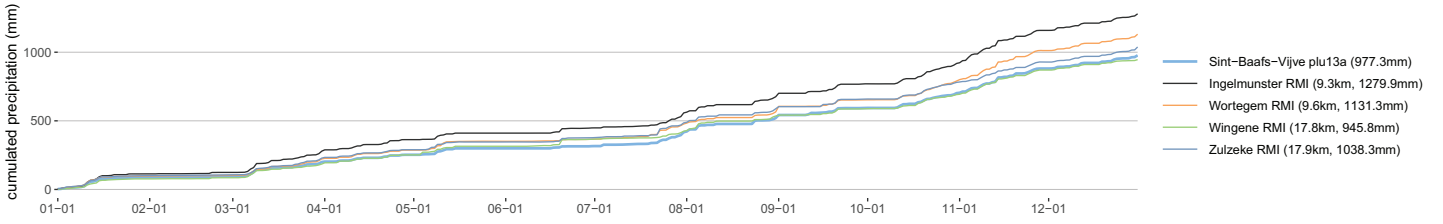
Sint-Baafs-Vijve plu13a monthly precipitation totals in 2023
