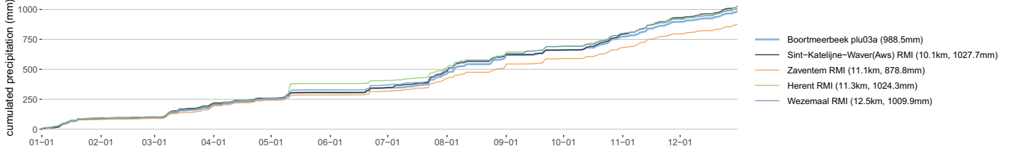
Boortmeerbeek plu03a cumulative precipitation in 2023
