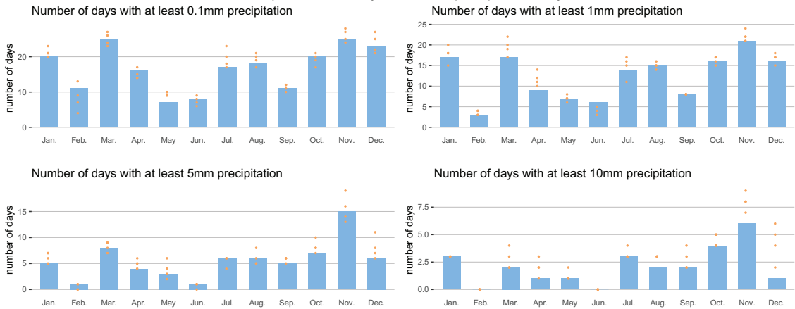
Sint-Laureins plu14a, monthly number of precipitation days in 2023
