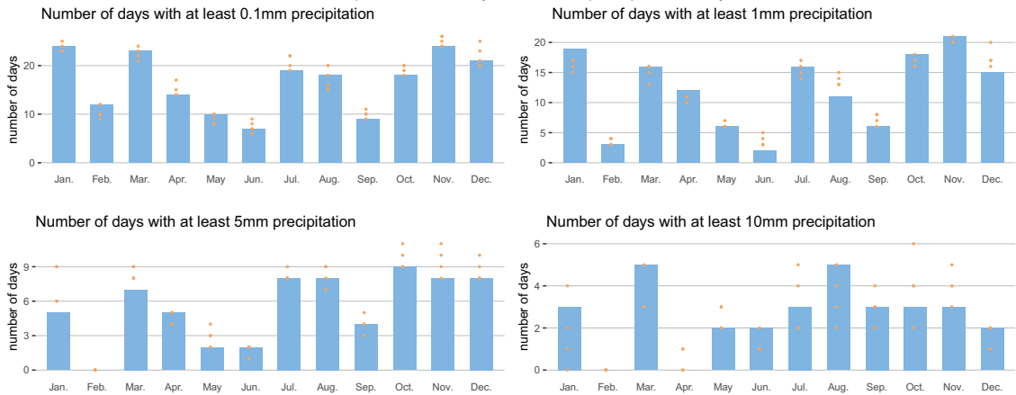
Boortmeerbeek plu03a, monthly number of precipitation days in 2023
