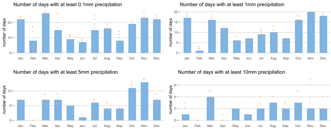
Ronse plu12a, monthly number of precipitation days in 2023
