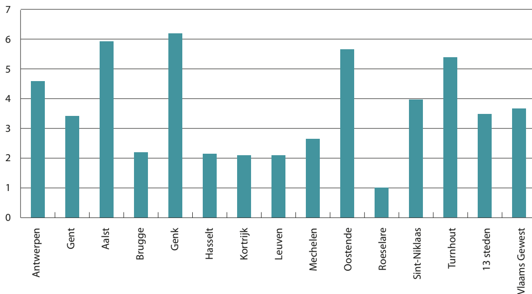
Spanningsindicator, in 2010, ratio.
