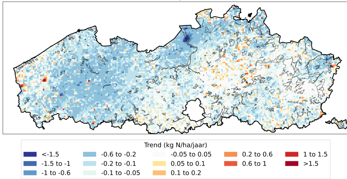
Totale Vlaamse \text{NH}_x -deposities Meteo 2017, VLOPS24
