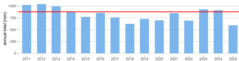
Ronse plu12a Time series of annual precipitation totals (blue bars) versus the climate normal 1991–2020 (horizontal line, 879mm)
