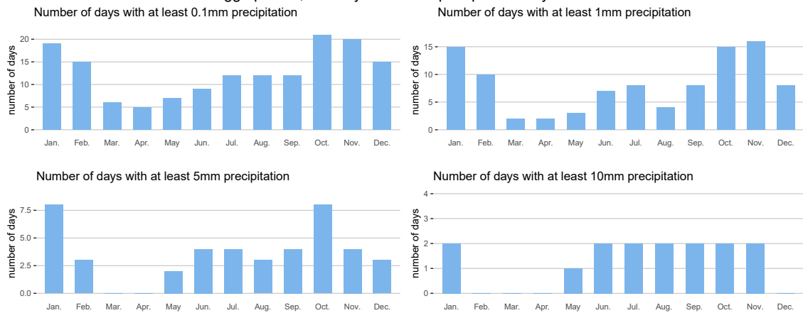
Brugge plu04a, monthly number of precipitation days in 2025
