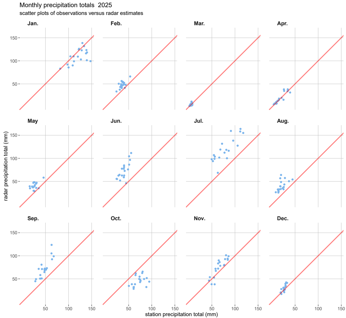
Figure 15: Scatter plots of the monthly totals of the HIC stations versus radar-derived estimates.
