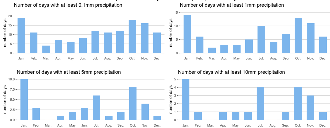
Boortmeerbeek plu03a, monthly number of precipitation days in 2025
