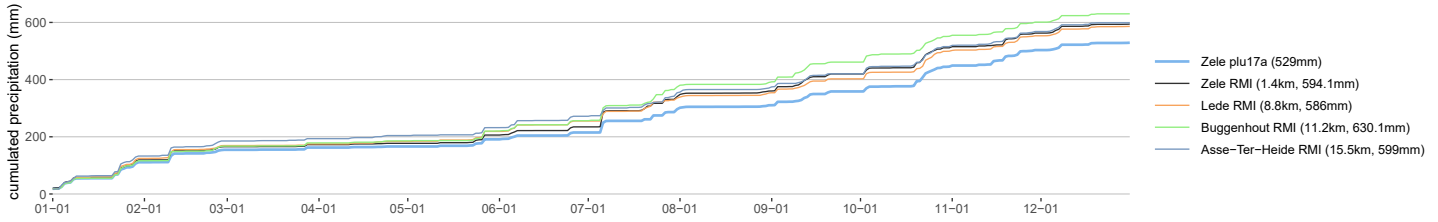
Zele plu17a cumulative precipitation in 2025
