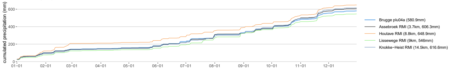
Brugge plu04a cumulative precipitation in 2025
