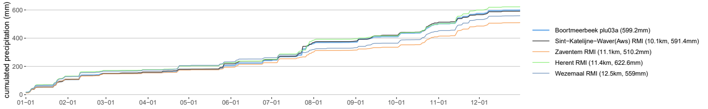
Boortmeerbeek plu03a cumulative precipitation in 2025
