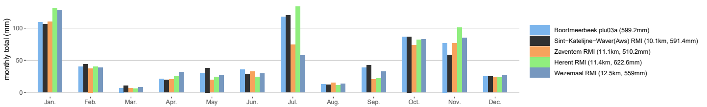
Boortmeerbeek plu03a monthly precipitation totals in 2025
