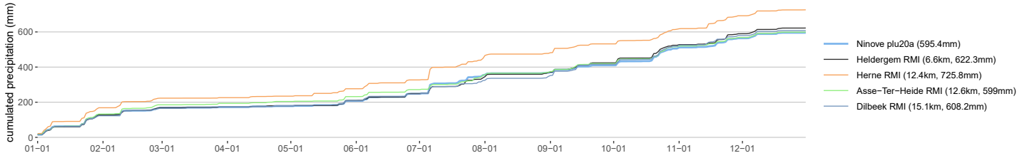
Ninove plu20a cumulative precipitation in 2025
