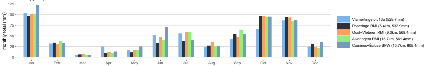
Vlamertinge plu16a monthly precipitation totals in 2025
