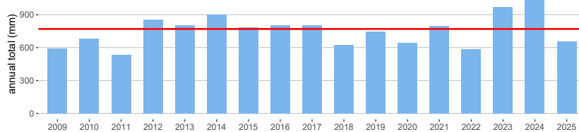
Time series of annual precipitation totals (blue bars) versus the climate normal 1991–2020 (horizontal line, 770mm)
