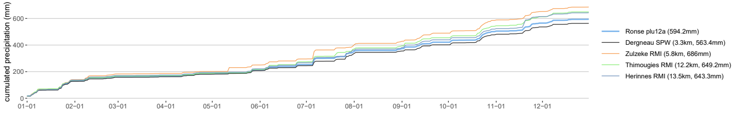
Ronse plu12a cumulative precipitation in 2025
