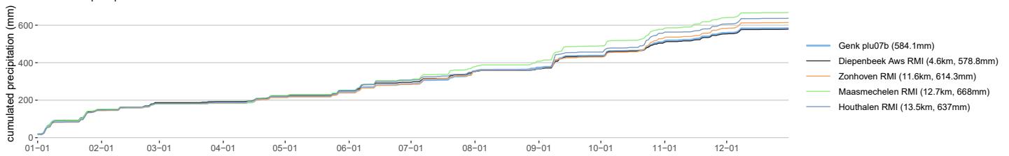
Genk plu07b cumulative precipitation in 2025
