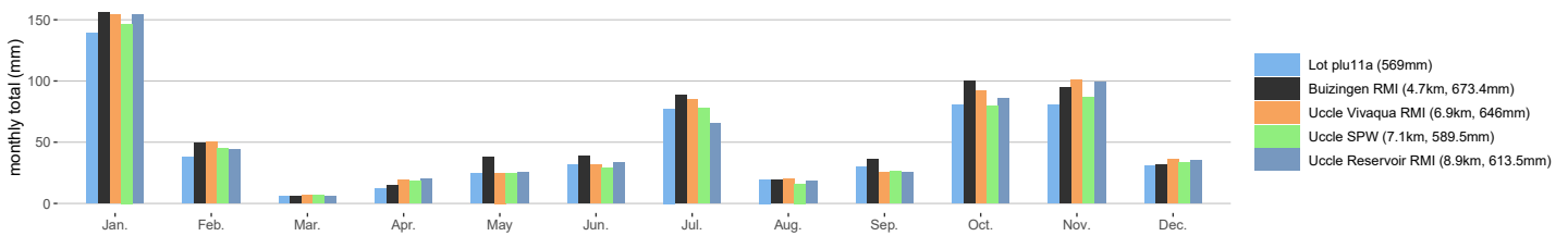
Lot plu11a monthly precipitation totals in 2025
