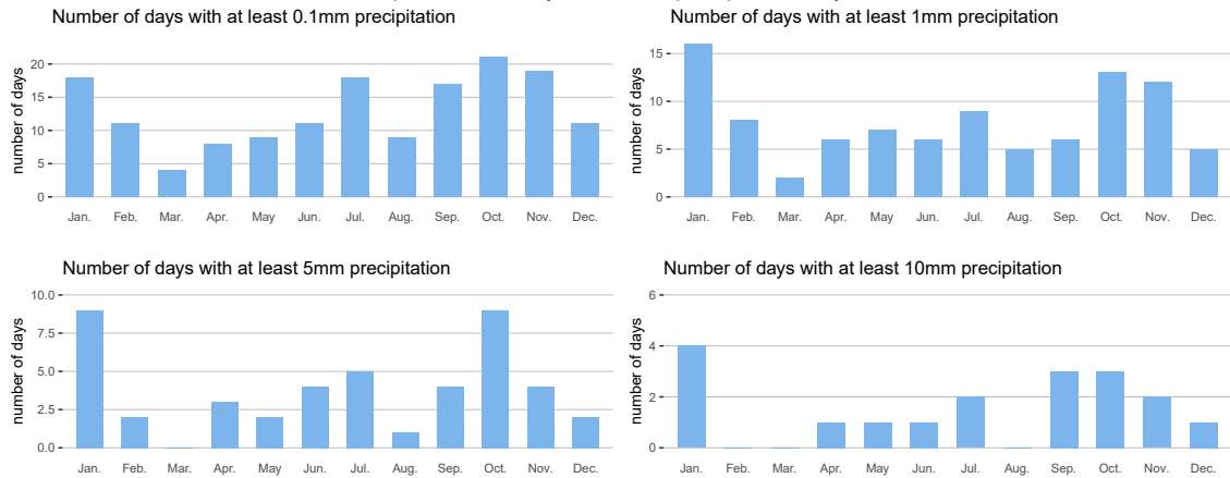
Lommel plu10a, monthly number of precipitation days in 2025
