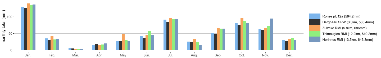
Ronse plu12a monthly precipitation totals in 2025
