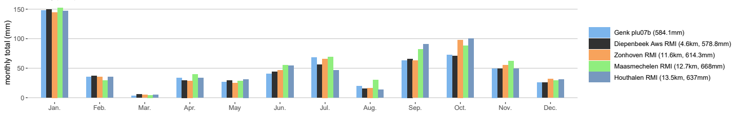
Genk plu07b monthly precipitation totals in 2025
