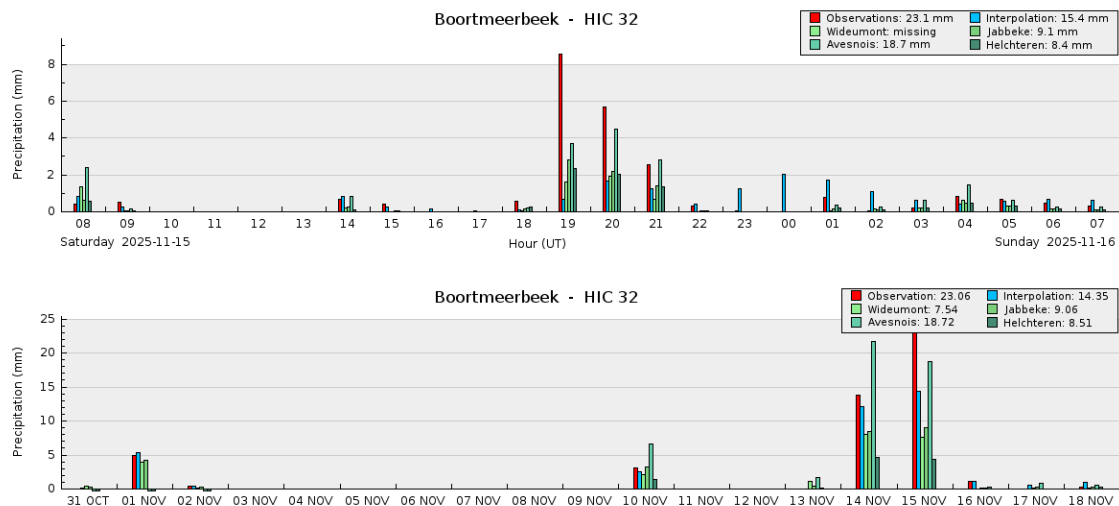
Figure 8: Comparison of hourly (top panel, case of November 15, 2025 for Boortmeerbeek) and daily (bottom panel, illustration of a period of 20 days including November 15, 2025 for Boortmeerbeek) data against an inverse distance weighing interpolation of neighboring stations and radar estimations.
