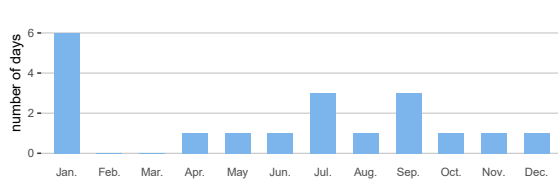
Number of days with at least 10mm precipitation
