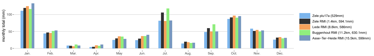
Zele plu17a monthly precipitation totals in 2025
