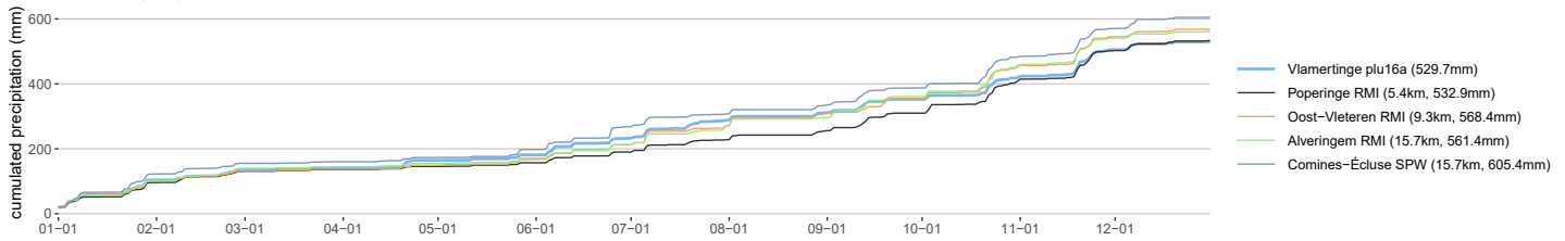
Vlamertinge plu16a cumulative precipitation in 2025
