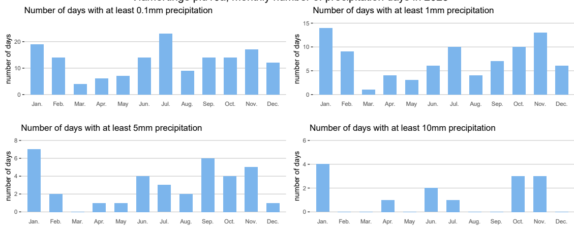
Vlamertinge plu16a, monthly number of precipitation days in 2025
