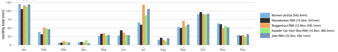
Bornem plu02a monthly precipitation totals in 2025
