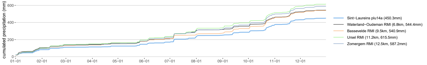
Sint-Laureins plu14a cumulative precipitation in 2025
