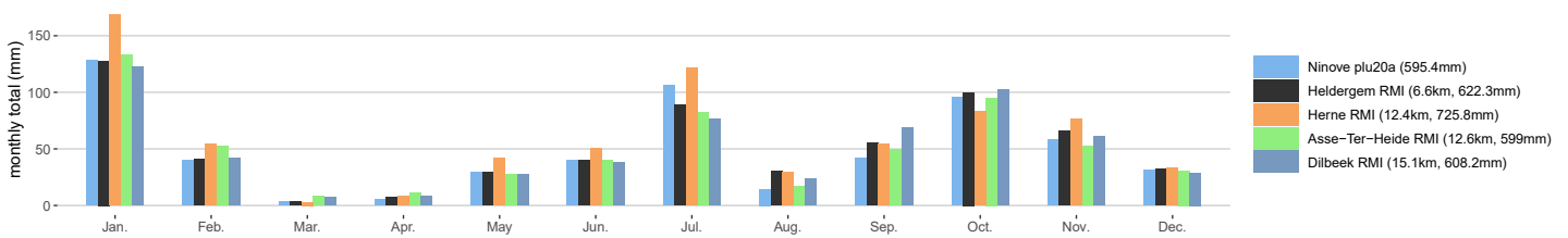
Ninove plu20a monthly precipitation totals in 2025
