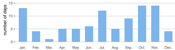
Number of days with at least 10mm precipitation
