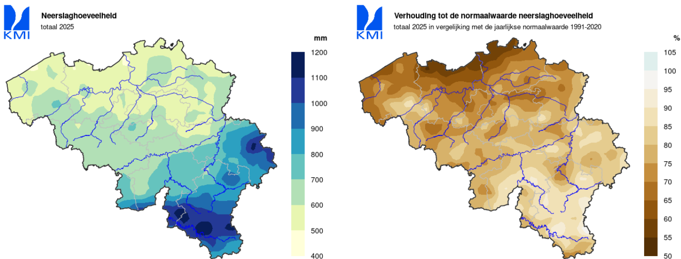
Figure 2: Map of the annual rainfall in Belgium in 2025 (left panel) and its deviation versus the 1991–2020 normal values (right panel). Local extremes are slightly smoothed in these maps.
