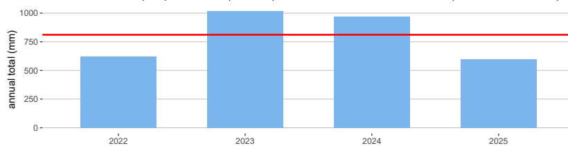
Time series of annual precipitation totals (blue bars) versus the climate normal 1991–2020 (horizontal line, 812mm)
