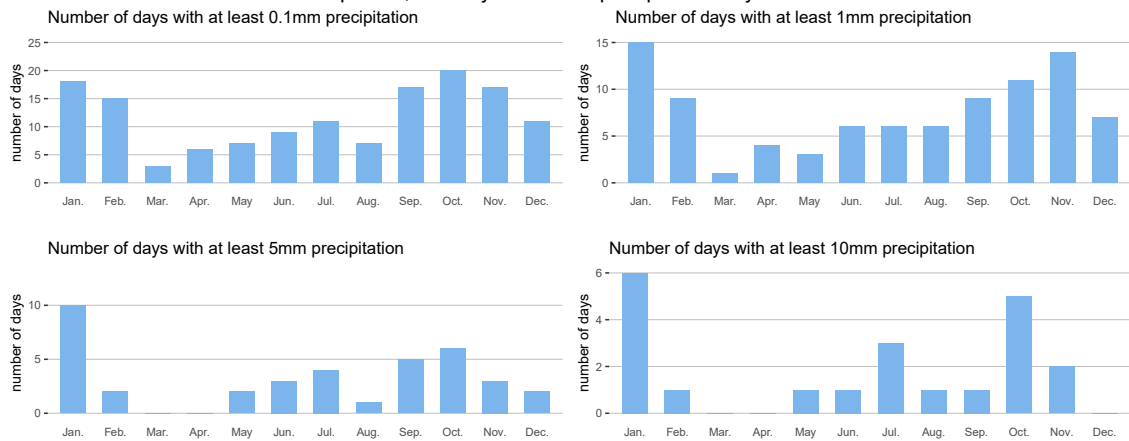
Elst plu06a, monthly number of precipitation days in 2025
