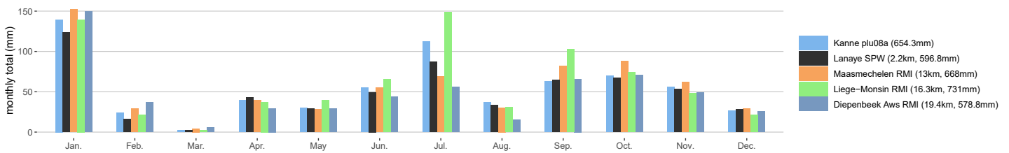
Kanne plu08a monthly precipitation totals in 2025
