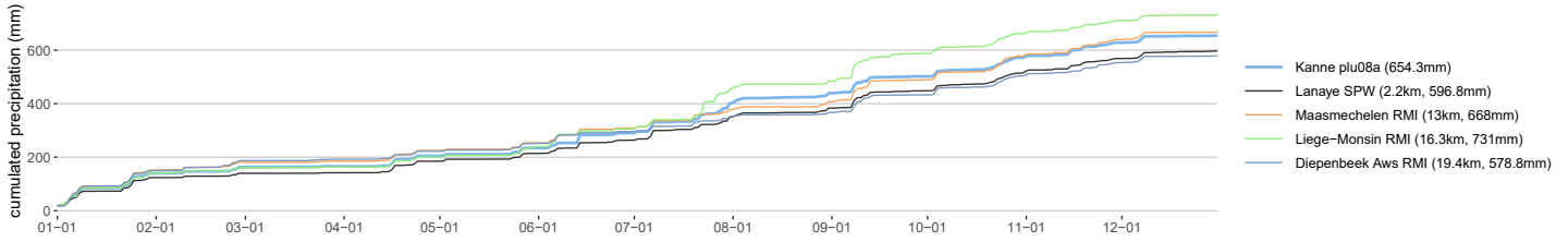
Kanne plu08a cumulative precipitation in 2025
