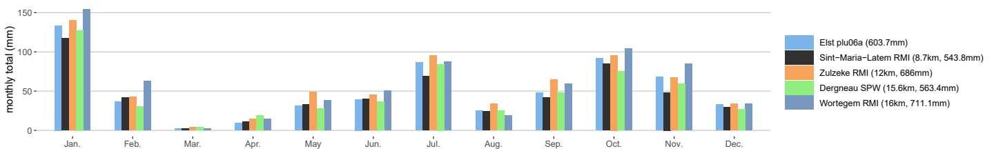
Elst plu06a monthly precipitation totals in 2025
