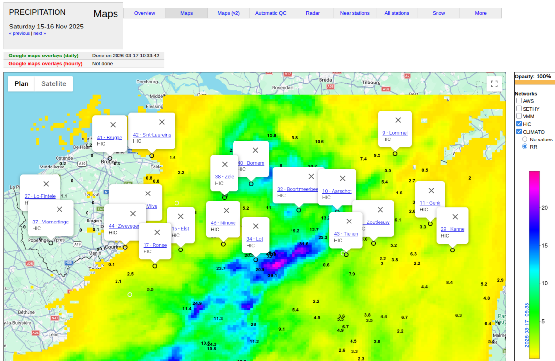
Figure 7: Data visualisation on maps in PluvioControl: comparison against daily radar data (case of November 15, 2025). The background field represents the estimations of the radar of Jabbeke. The numbers correspond to the observations of the climatological stations.
