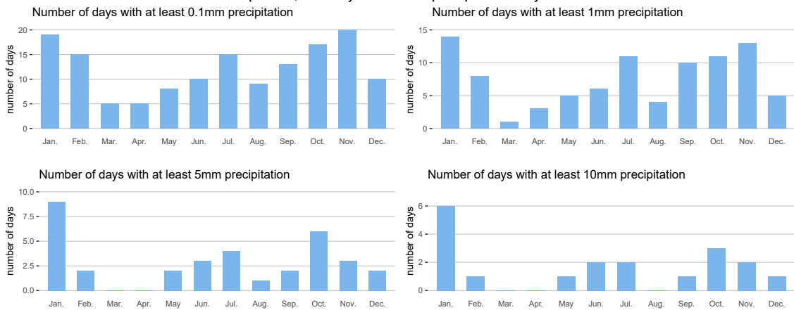
Ninove plu20a, monthly number of precipitation days in 2025
