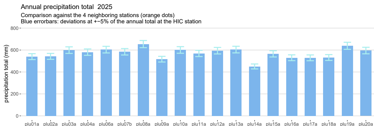
Figure 11: Comparison of the annual total of the HIC stations against the corresponding values of the 4 closest rain gauges (orange dots).
