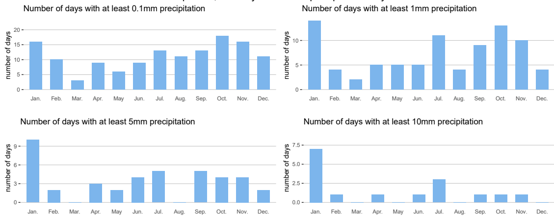
Zoutleeuw plu18a, monthly number of precipitation days in 2025
