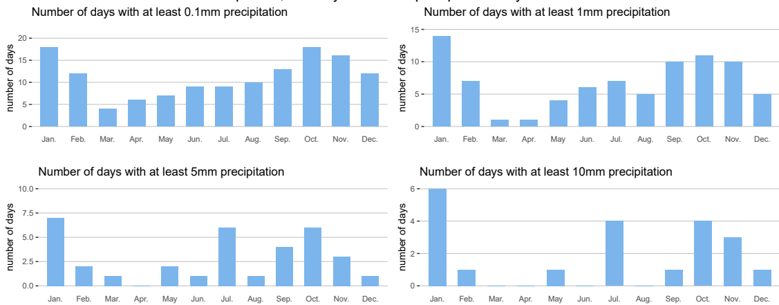
Zele plu17a, monthly number of precipitation days in 2025
