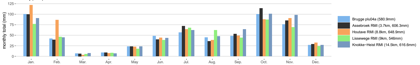
Brugge plu04a monthly precipitation totals in 2025
