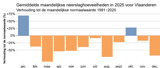
Figure 3: Monthly precipitation anomalies with respect to the period 1991–2020 on average for the Flemish Region from January to December 2025.
