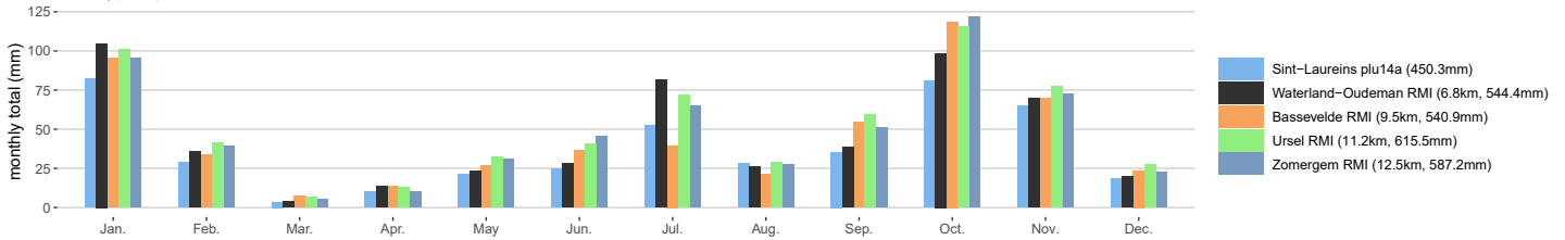
Sint-Laureins plu14a monthly precipitation totals in 2025
