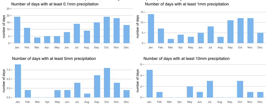
Bornem plu02a, monthly number of precipitation days in 2025
