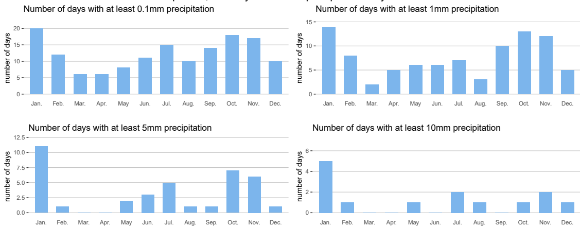
Lot plu11a, monthly number of precipitation days in 2025
