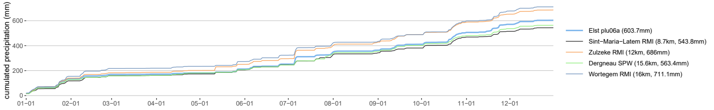
Elst plu06a cumulative precipitation in 2025
