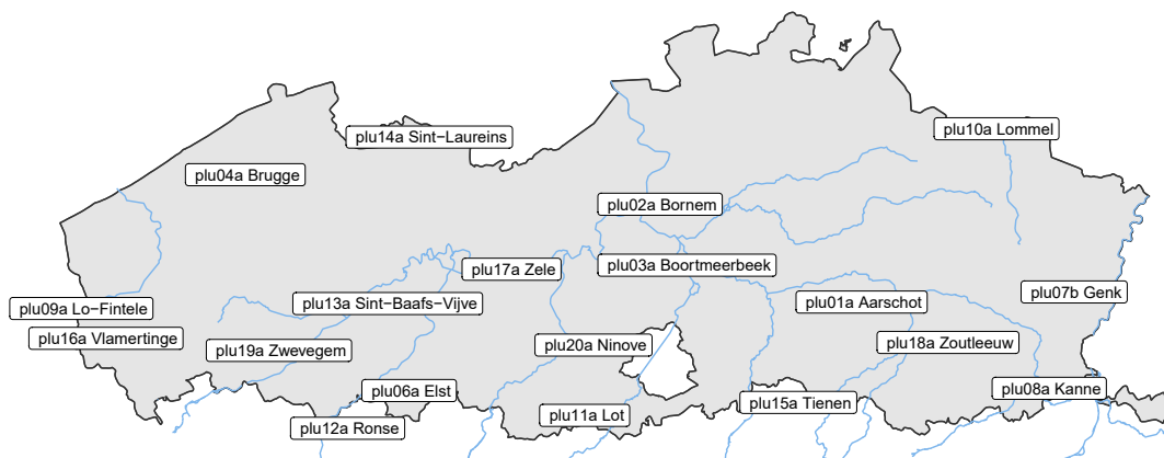
Figure 5: Location of the operational HIC rain gauges in 2025.
