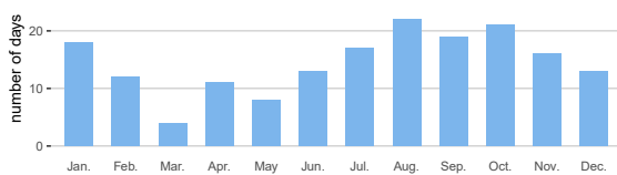
Number of days with at least 5mm precipitation
