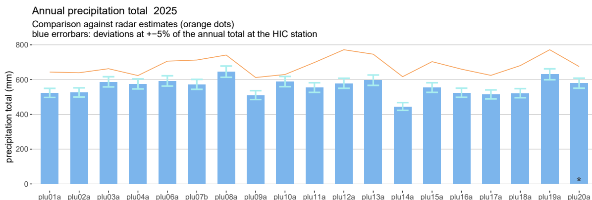
Figure 13: Comparison of the annual total of the HIC stations against radar-derived estimates.
