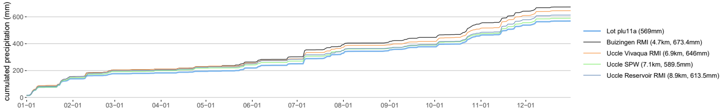
Lot plu11a cumulative precipitation in 2025
