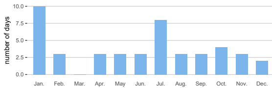
Number of days with at least 5mm precipitation
