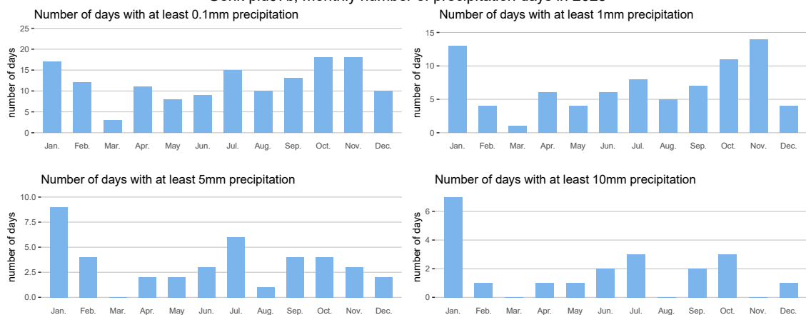
Genk plu07b, monthly number of precipitation days in 2025
