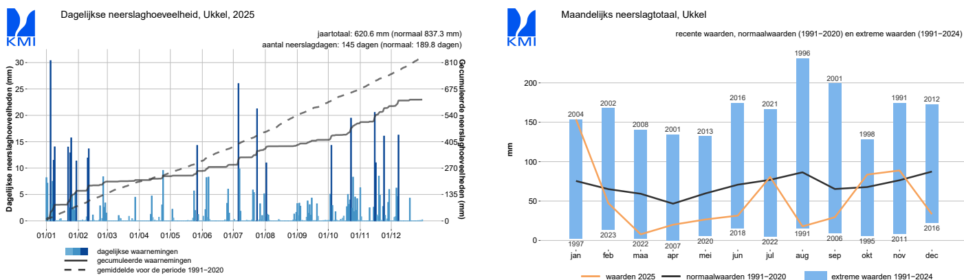
Figure 1: Daily and monthly precipitation values in Uccle in 2025.
