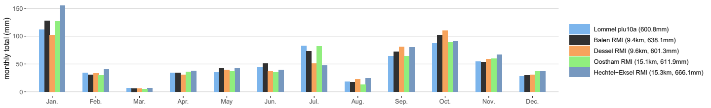
Lommel plu10a monthly precipitation totals in 2025
