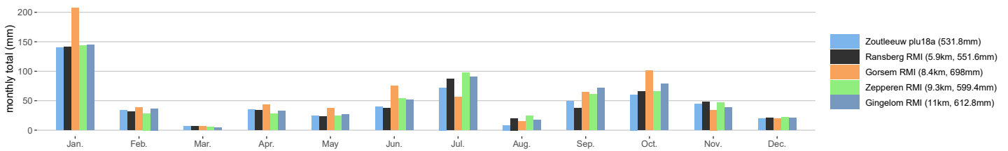
Zoutleeuw plu18a monthly precipitation totals in 2025
