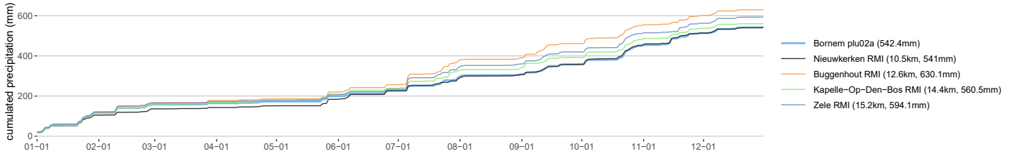
Bornem plu02a cumulative precipitation in 2025
