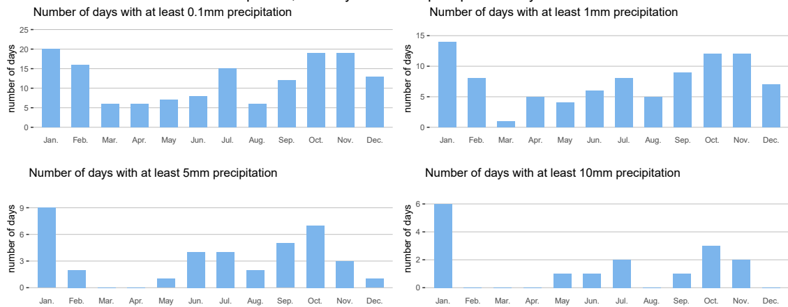
Ronse plu12a, monthly number of precipitation days in 2025
