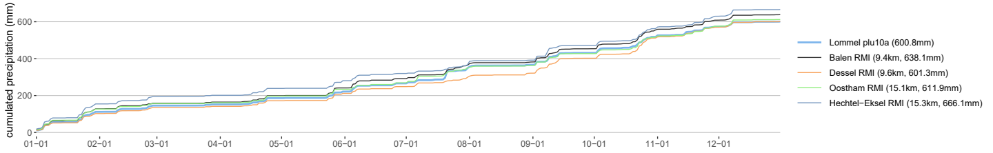
Lommel plu10a cumulative precipitation in 2025
