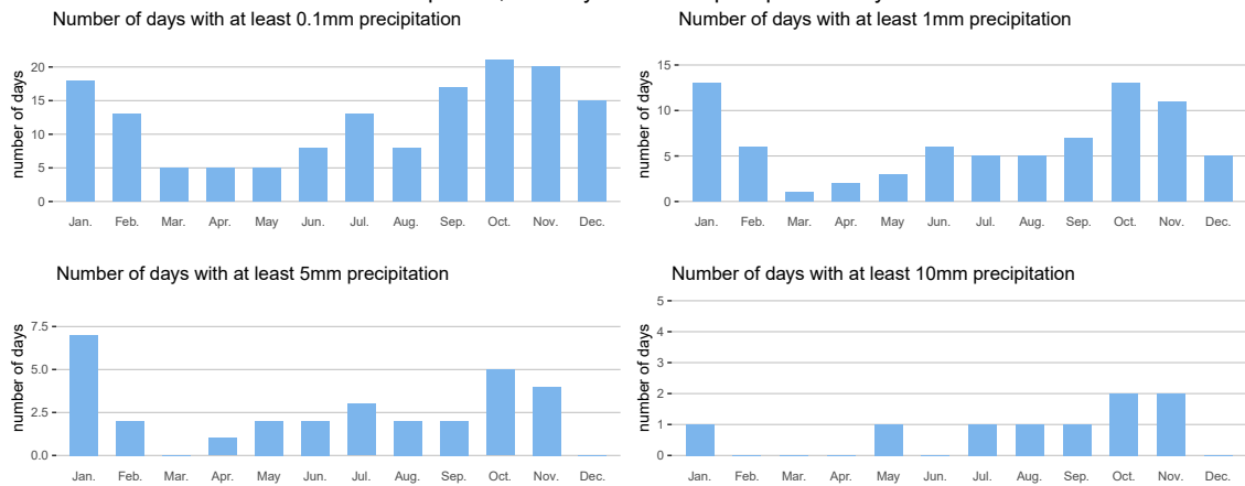
Sint-Laureins plu14a, monthly number of precipitation days in 2025
